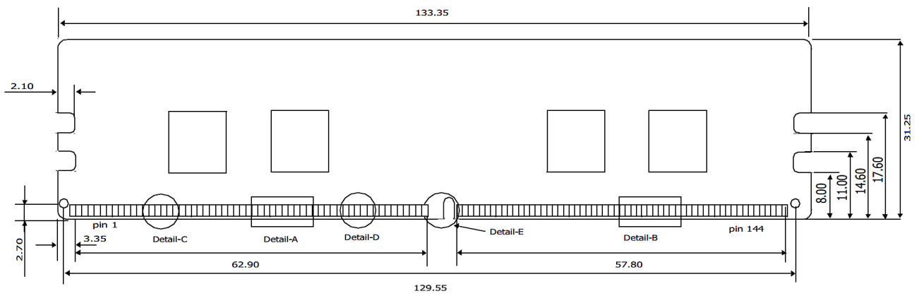
Front view
